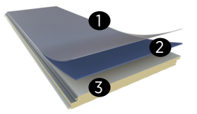
AW2500 PVDF-Coastal Standard Coastal Finish ① .75 mil nominal top coat ② 1.1 nominal primer ③ Substrate
