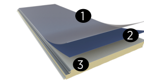
AW100 Polyester Standard Interior Finish ① .75 mil nominal top coat ② .25 mil nominal primer ③ Substrate
