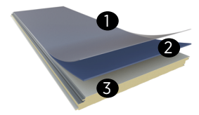
AW2000/2250 PVDF/FEVE-High Build High Build Exterior Finish ① .75 mil nominal top coat ② 1.0 mil nominal primer ③ Substrate
