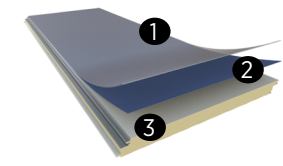
AW250 AdobeTexture® Stucco Finish ① .8 mil nominal top coat ② .2 mil nominal primer ③ Substrate
