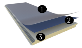
AW500 SMP Solid Color Exterior Finish ① .75 mil nominal top coat ② .25 mil nominal primer ③ Substrate
