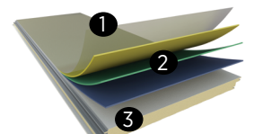
AW4500 PVDF-Coastal High Build Coastal Finish ① .75 mil nominal top coat ② 3 coats 1.0 mil nominal primer ③ Substrate
