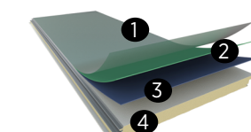
AW3000/3250 PVDF/FEVE-Metallic Exterior Metallic with Clear Coat ① .50 mil nominal clear coat ② .75 mil nominal top coat ③ .2 mil nominal primer ④ Substrate
