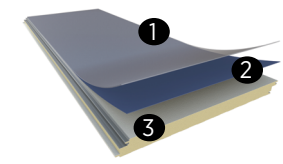
AW1500/1750 PVDF/FEVE-Mica Exterior Finish with Iridescent Shine ① .75 mil nominal top coat ② .25 mil nominal primer ③ Substrate
