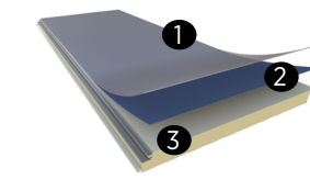
AW1000/1250 PVDF/FEVE High Performance Exterior Coating ① .75 mil nominal top coat ② .25 mil nominal primer ③ Substrate
