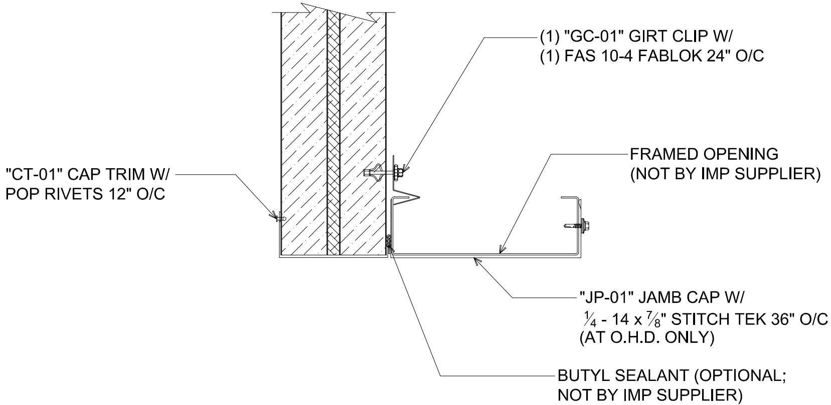
# FRAMED OPENING JAMB (PLAN VIEW )
