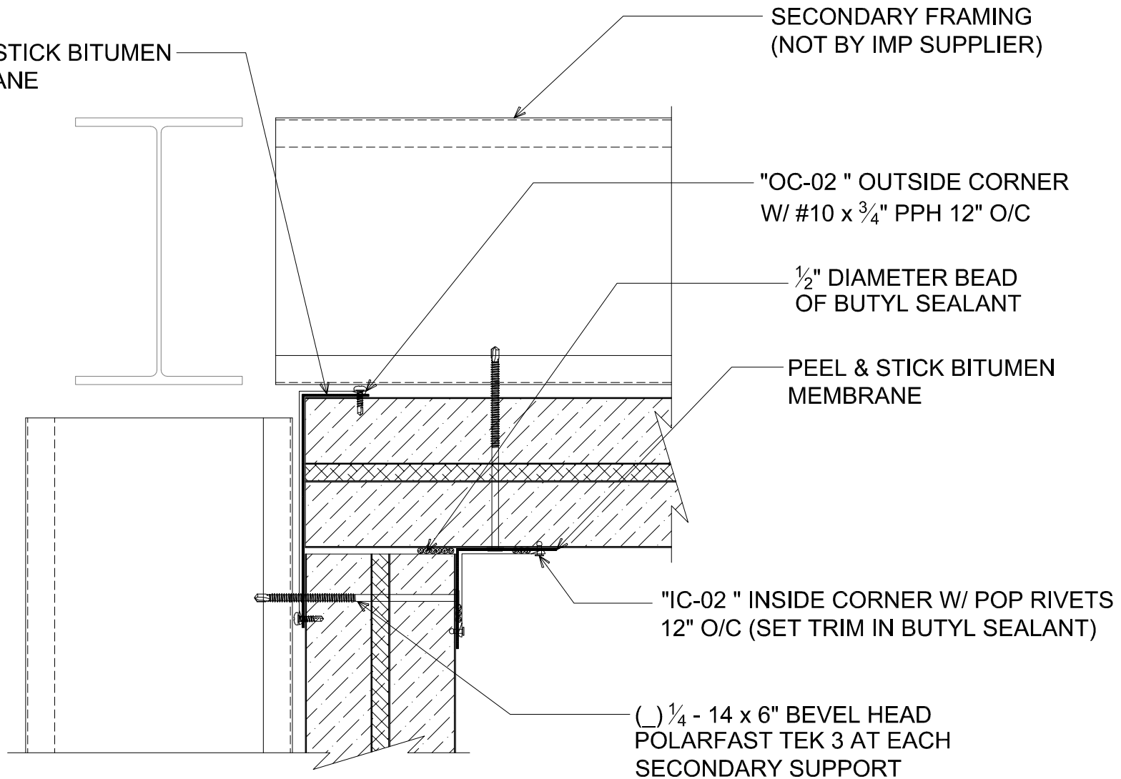
# CORNER TRANSITION - FLAT INSIDE (PLAN VIEW)
