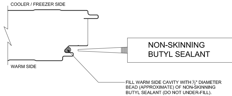
SEALANT PLACEMENT AT PANEL JOINT (PLAN VIEW - EXTERIOR WALL)
