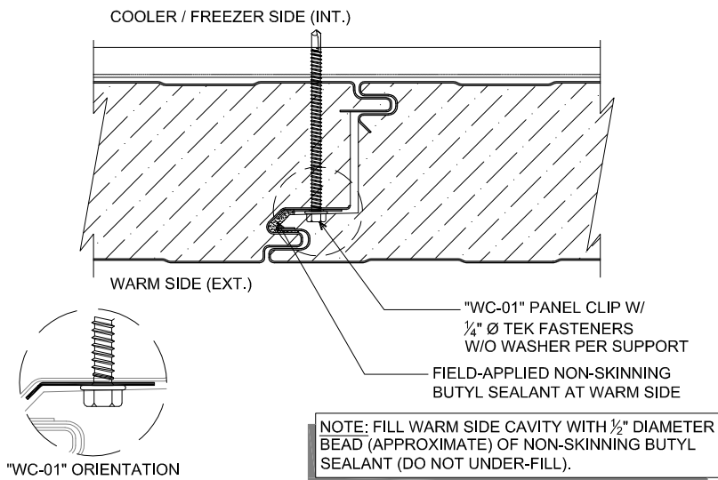
PANEL JOINT (COLD-STORAGE) (PLAN VIEW - EXTERIOR WALL)
