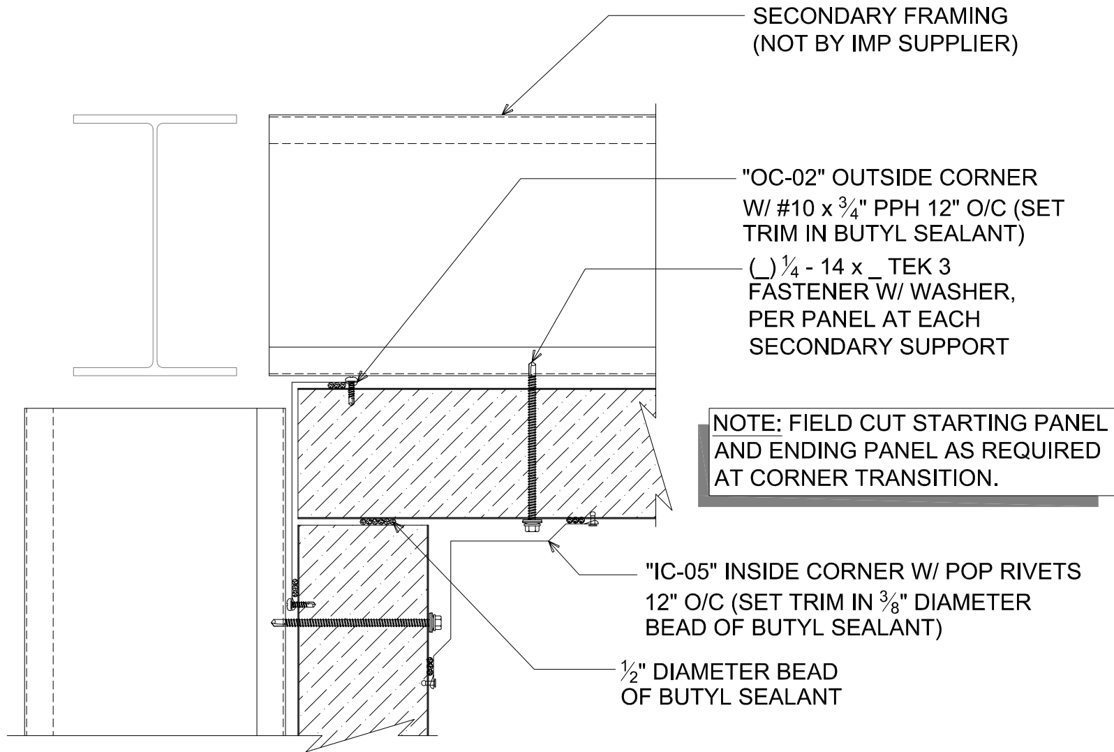
# CORNER TRANSITION - SCULPTED INSIDE (PLAN VIEW)
