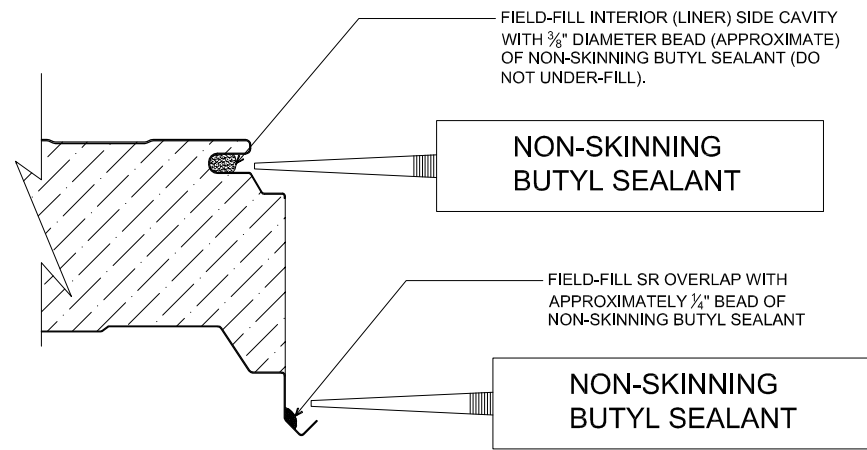
SEALANT PLACEMENT AT PANEL JOINT
